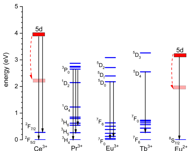
Fig. 2 Relevant level energies and luminescence transitions of \text{Ce}^{3+} , \text{Pr}^{3+} , \text{Eu}^{3+} , \text{Tb}^{3+} , and \text{Eu}^{2+} . The energy of the lowest 5d -level depends on the compound and the range is indicated by the curved dashed arrows.
