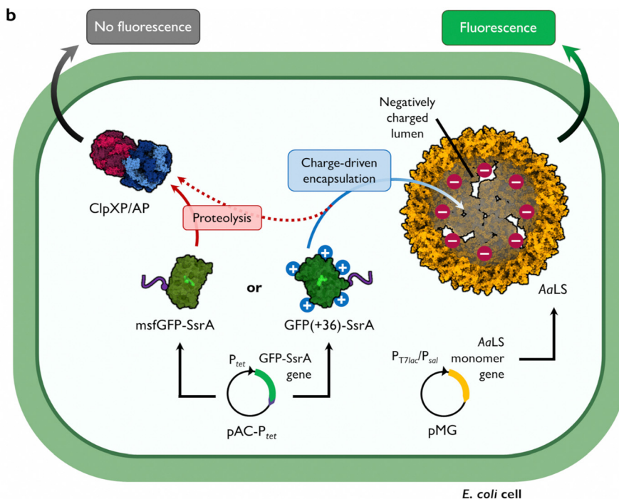
Fig. 1 Shield-or-shred system: in cellulo ionic interaction-based guest encapsulation of otherwise degradation-prone fluorescent protein by engineered Aquifex aeolicus lumazine synthase (AaLS) protein cages. (a) Structures of AaLS-wt 60-mer (PDB: 5MPP), AaLS-neg 180-mer (5MQ3), AaLS-13 360-mer (5MQ7). Scale bar – 20 nm. Electrostatic potential molecular surfaces (Connolly representation, upscaled 3×) of the pentameric subassemblies, projected perpendicularly to the five-fold symmetry axis, viewed from the luminal face, are shown next to the respective cages. 20–22 (b) Conceptual scheme of the in cellulo guest encapsulation experiments. A GFP fused to SsrA degron peptide, either non-supercharged (msfGFP-SsrA) or positively supercharged (GFP(+36)-SsrA), is coproduced in E. coli cells with a selected protein cage and its fluorescence is analysed. Models are not to scale.
