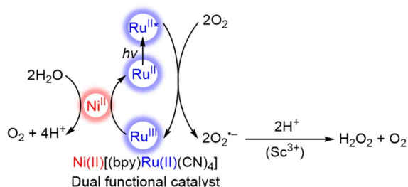
Scheme 2 Catalytic mechanism for the formation of hydrogen peroxide from water and dioxygen with a dual functional catalyst, Ni(II) [(bpy)Ru(II)(CN)_4] , under visible light irradiation. 71
