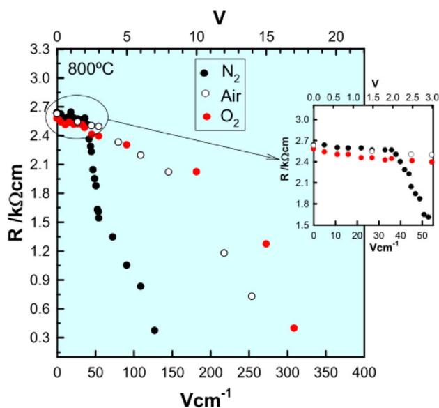
Fig. 5 Resistance of Y_{0.5}Zr_{0.49}Mg_{0.01}O_{1.74} as a function of bias voltage at 800 °C in different atmospheres; reproduced from M. Jovani et al. , Sci. Rep. , 2019, 9, 18538, with permission from Springer Nature.
