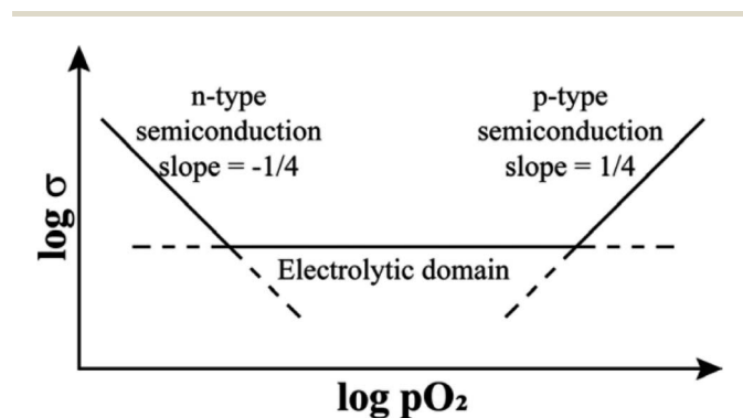
Fig. 1 Schematic ionic and electronic conductivity domains as a function of pO 2 .
