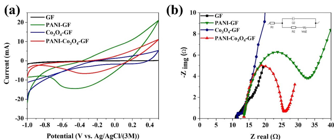
Fig. 4 Electrochemical characterisation of the anode electrodes before use. (a) CV scans at 0.01 V \text{s}^{-1} and (b) EIS spectra. Tests were performed in a 3-electrode system in 50 mM PBS (pH 7), with the anode as the working electrode and Pt wire (diameter: 0.127 mm) as the counter electrode.
