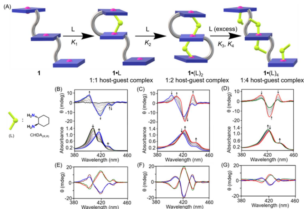
Fig. 2 (A) Schematic representation of the formation of 1 : 1, 1 : 2 and 1 : 4 host–guest complexes between 1 and \text{CHDA}_{(R,R)} . CD and UV spectral changes (in \text{CH}_2\text{Cl}_2 at 295 K) of 1 (at 3 \times 10^{-6} M) upon addition of \text{CHDA}_{(R,R)} as the host–guest molar ratio changes from (B) 1 : 0 to 1 : 50, (C) 1 : 50 to 1 : 500 and (D) 1 : 500 to 1 : 4000. Calculated (cal) and observed (obs) CD spectra (E) of 1 \cdot \text{CHDA}_{(R,R)} (brown, cal), 1 \cdot \text{CHDA}_{(S,S)} (green, cal), 1 \cdot \text{CHDA}_{(R,R)} (blue, obs) and 1 \cdot \text{CHDA}_{(S,S)} (red, obs); (F) 1 \cdot (\text{CHDA}_{(R,R)})_2 (brown, cal), 1 \cdot (\text{CHDA}_{(S,S)})_2 (green, cal), 1 \cdot (\text{CHDA}_{(R,R)})_2 (blue, obs) and 1 \cdot (\text{CHDA}_{(S,S)})_2 (red, obs); and (G) 1 \cdot (\text{CHDA}_{(R,R)})_4 (brown, cal), 1 \cdot (\text{CHDA}_{(S,S)})_4 (green, cal), 1 \cdot (\text{CHDA}_{(R,R)})_4 (blue, obs) and 1 \cdot (\text{CHDA}_{(S,S)})_4 (red, obs).
