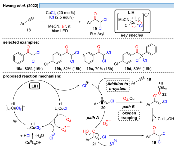
Scheme 6 Synthesis of α-keto-dichlorination of arylalkynes.
