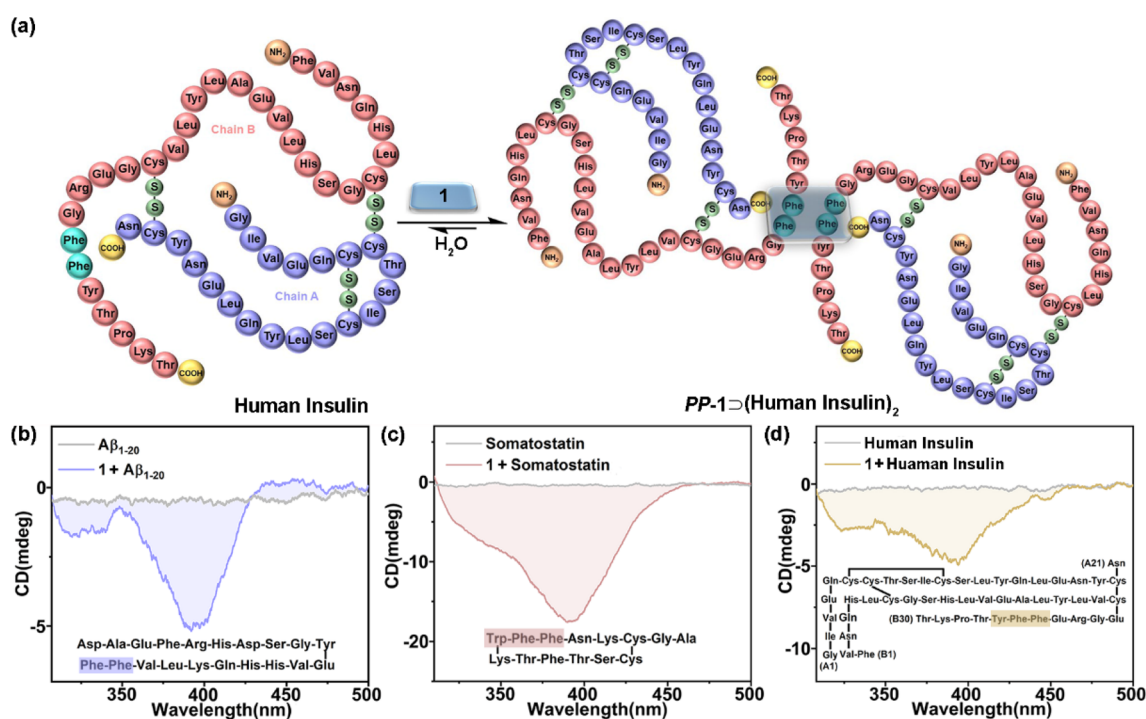
Fig. 5 (a) Schematic representation of a possible binding model of 1 ⊃(human insulin) 2 . CD spectra of 1 (20 \mu\text{M} ) with (b) \text{A}\beta_{1-20} (2.0 equiv.), (c) somatostatin (2.0 equiv.), and (d) human insulin (1.0 equiv.) in phosphate buffer (10 mM sodium phosphate, pH = 7.4). (Inset) The possible binding sites.
