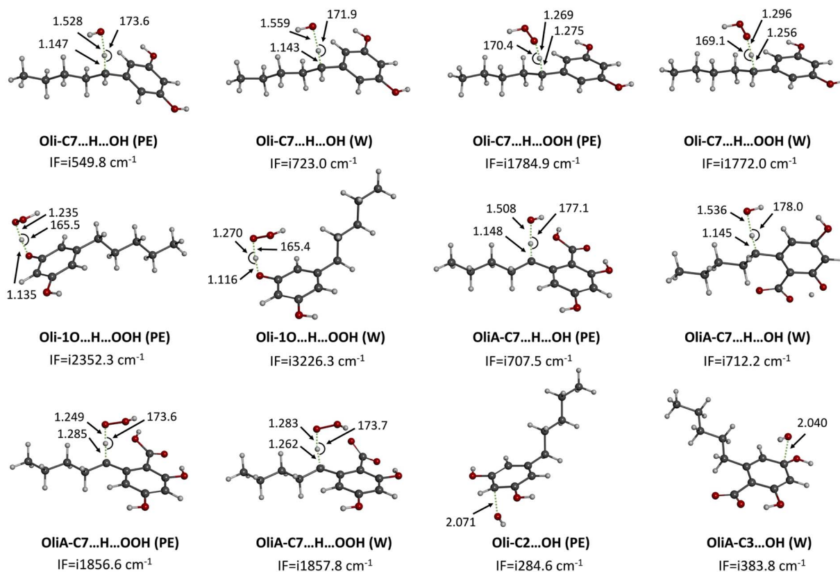
Fig. 4 Localized TSs of the reaction of Oli and OliA with HO • and HOO • under physiological conditions. IF = imaginary frequencies, W = water, and PE = pentyethanoate.
