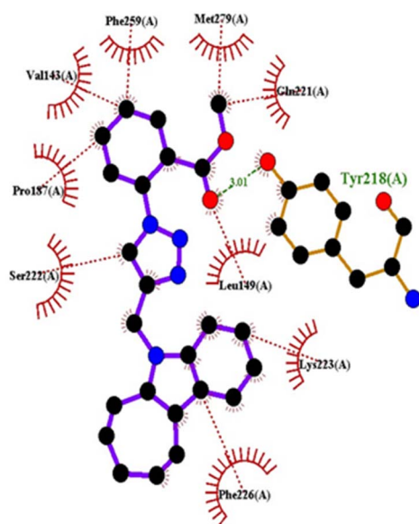
Fig. 13 2D interactions of compound 4h with 1FDW.
