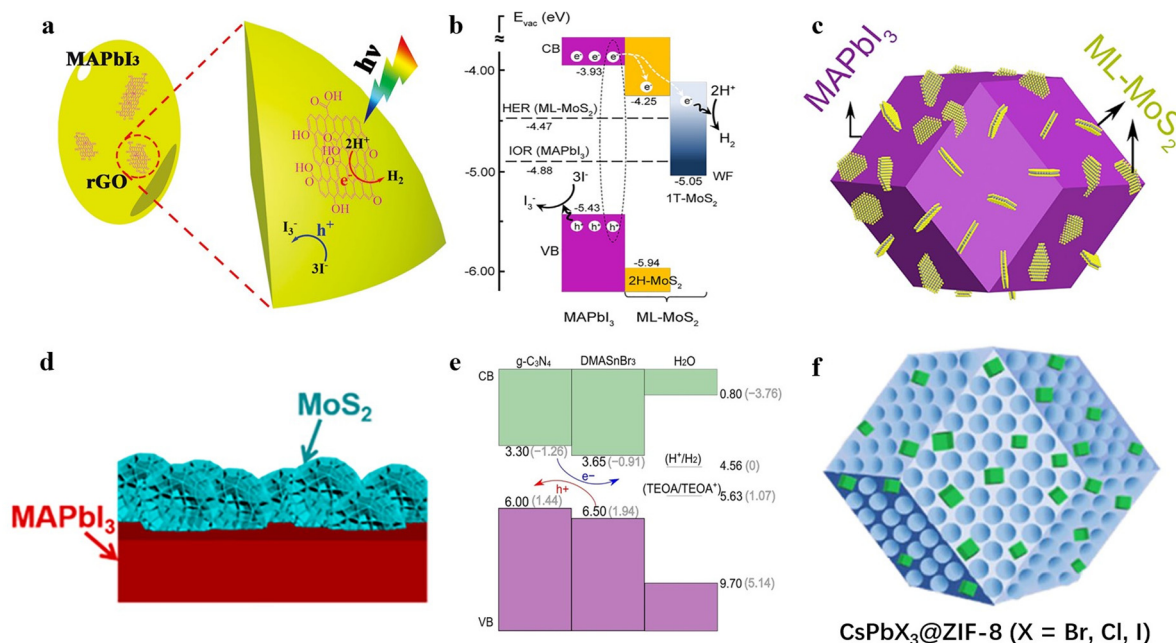
Fig. 10 (a) The schematic diagram of photocatalytic HER on MAPbI 3 /rGO. 115 Copyright 2018 Wiley-VCH GmbH. (b) The schematic diagram of photocatalytic HER on ML-MoS 2 /MAPbI 3 -MCs. 126 Copyright 2020 Elsevier. (c) The schematic illustration of structure of ML-MoS 2 /MAPbI 3 -MCs. 126 Copyright 2020 Elsevier. (d) The schematic illustration of structure of MoS 2 nanoflowers/MAPbI 3 microcrystals. 131 Copyright 2021 American Chemical Society. (e) The schematic mechanism of photocatalytic HER on g-C 3 N 4 /DMASnBr 3 /Pt in triethanolamine solution. 128 Copyright 2018 Wiley-VCH GmbH. (f) The schematic illustration of structure of CsPbX 3 @ZIF-8 (X = Br, Cl, I). 135 Copyright 2022 American Chemical Society.
