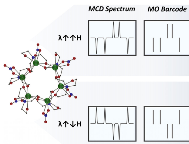
Scheme 1 (Left) Crystal structure of [\text{Er}_6(\text{teaH})_6(\text{NO}_3)_6] \cdot 6\text{H}_2\text{O} , \{\text{Er}_6\} (colour code: green (Er); red (O), blue (N), black (C)) MCA (CCDC number: 1876163). (Right) representation of the dual-signalled magneto-optical barcode obtained via MCD spectroscopy.
