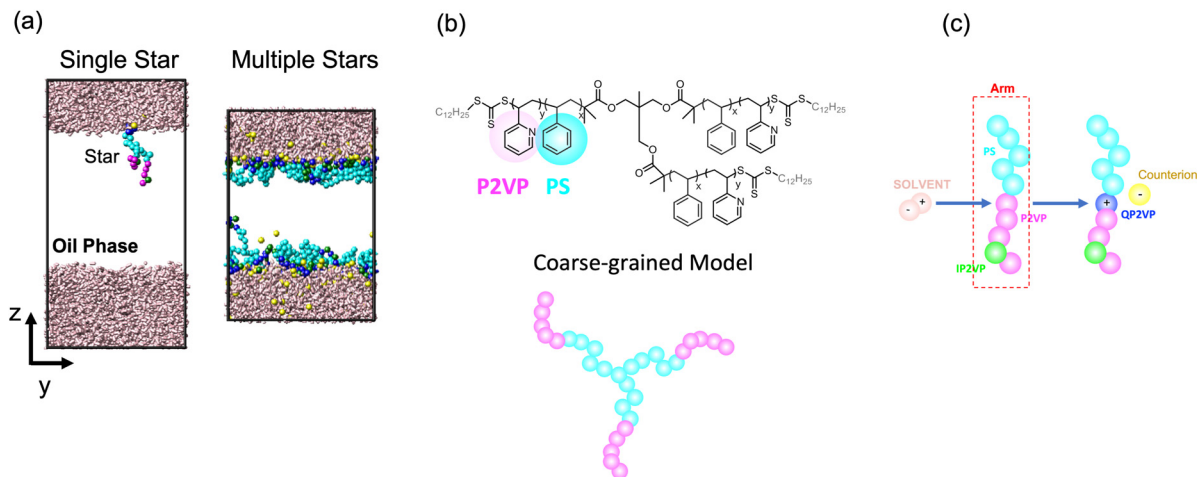
Fig. 1 Simulation box showing a single star or multiple stars at the dielectric solvent-oil interface (a). Cyan beads are lyophilic beads representing PS, blue beads are quarternized P2VP or QP2VP, green beads are inert P2VP beads or IP2VP, pink rods are dielectric solvent molecules representing the aqueous phase and oil beads are not shown for clarity. Atomistic and coarse-grained representation of a 3-arm PS-P2VP block copolymer star (b). Ad hoc protonation reaction where a dipolar solvent molecule is consumed when the positively charged end of the solvent molecule comes into contact with a P2VP bead (within a 1.3\sigma cutoff). The P2VP bead is quarternized to QP2VP, which is positively charged, and a counterion is dissociated (c). Movies of the systems shown in (a) illustrating the ad hoc protonation reaction and the assembly of stars at the interface are provided in the ESI.†
