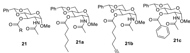
Fig. 13 C-3 ester derivatives of N -acetyl-D-glucosamines.
