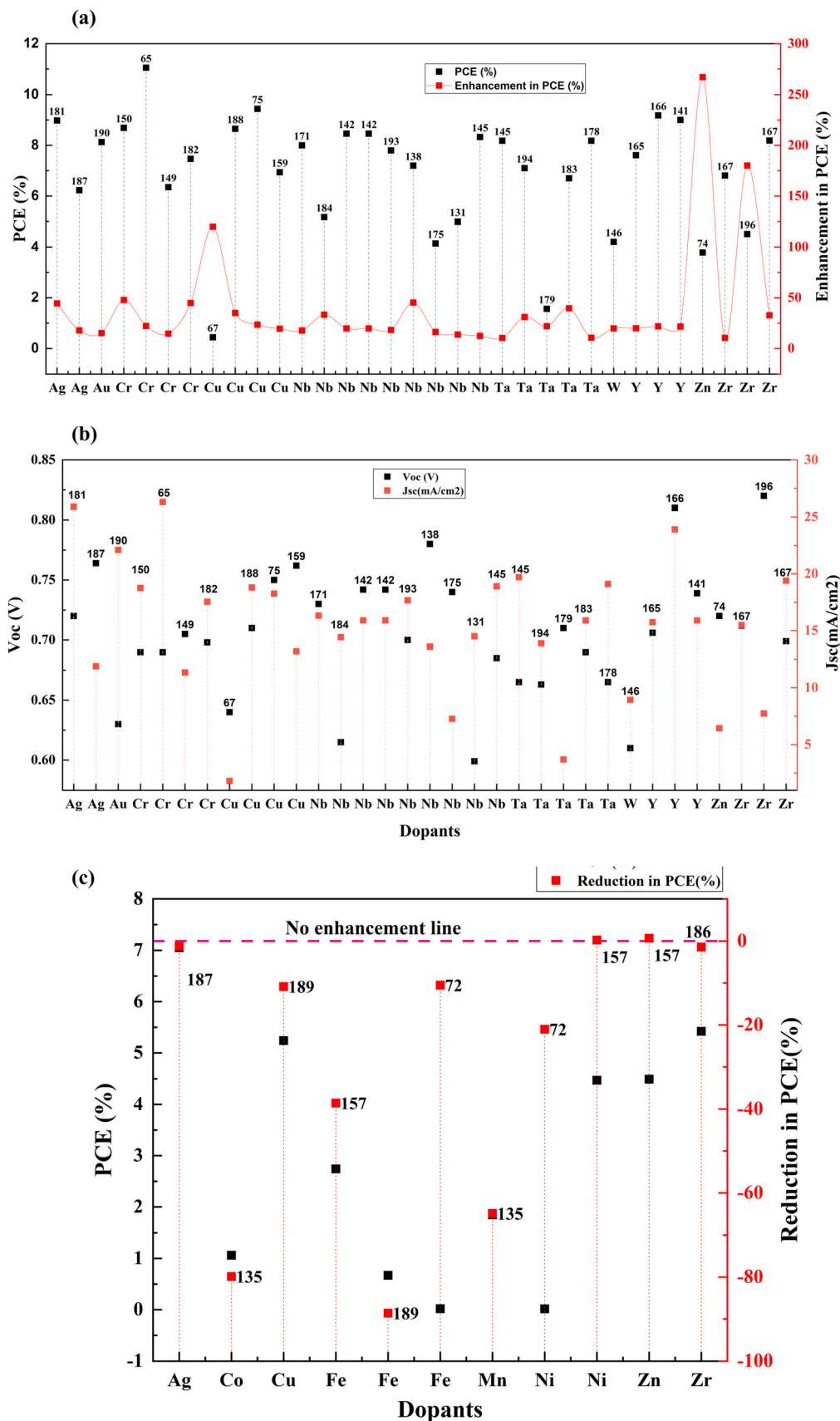
Fig. 21 (a) Performance of transition metals when doped into \text{TiO}_2 for DSSC fabrication. (b) J_{sc} and V_{oc} of transition metals when doped into \text{TiO}_2 for DSSC fabrication. (c) Reduction in PCE when transition elements are doped into \text{TiO}_2 for DSSC fabrication. Data points are labelled with references.
