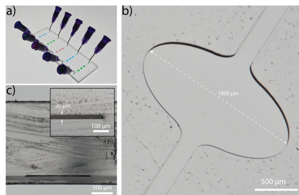
Fig. 2 a) Photograph of a sealed and connected chip incorporating five individual channels. b) Focus stack image of the imprinted channel structure into 240\ \mu\text{m} thick COC. c) Image of the cross-section of a microfluidic channel sealed with a 2\ \text{mm} thick COC slide by the solvent-assisted bonding technique (the inset shows the channel at higher resolution).
