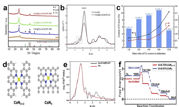
Fig. 10 (a) XRD patterns of CoO@Co–N–bCNT samples synthesized at different temperatures. 80 (b) Co K-edge EXAFS spectra of CoO@Co–N–bCNT-8:2 (8:2 is mass ratio of Co source to melamine) and Co foil. 80 (c) Relationship among E_{1/2} , N content and Co content of the CoO@Co–N–bCNT samples. 80 (d) Structure of CoN 2+2 and CoN 4 active sites. 84 (e) The fitted spectra of FT-EXAFS for the Co–N–C@F127 catalyst. 84 (f) Free energy evolution diagram for the 4e - ORR pathway on the CoN 2+2 and CoN 4 active sites. 84
