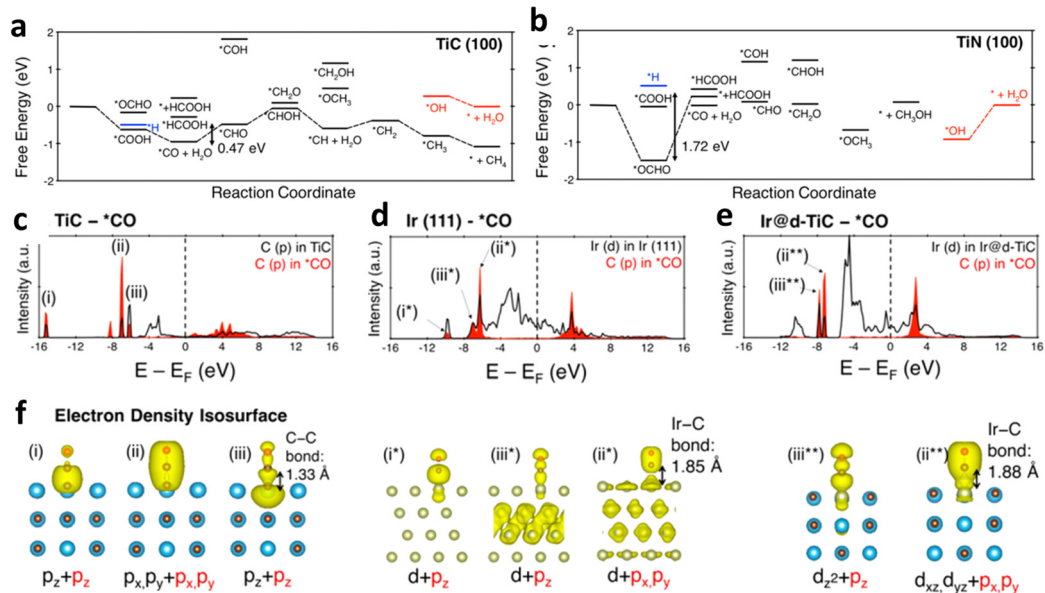
Fig. 11 Free-energy profiles for ECR on (a) TiC and (b) TiN. Density of states of (c) TiC, (d) Ir, and (e) Ir@d-TiC interacting with ^*CO . (f) The electron density isosurfaces at noted panels of (c)–(e). Reproduced with permission. 88 Copyright (2017) American Chemical Society.
