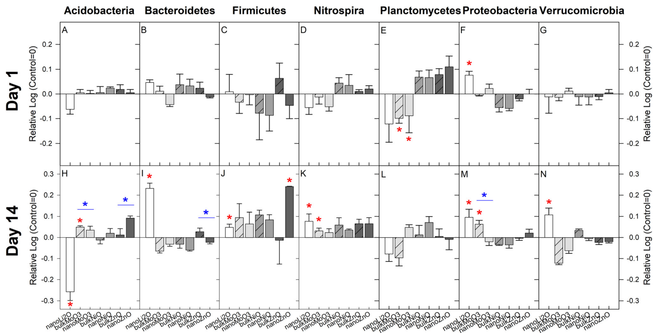
Fig. 1 Differential abundance analysis of prokaryotic (16S rDNA gene V4) phyla in soils at 1 (A–G) and 14 (H–N) days after metal oxide application. Control was soil with no metal oxide addition. Logarithm (base 10) of the relative response ( i.e. , soil response to metal oxide/response of soil control) are presented, where positive and negative numbers represent an increase or decrease in activity, respectively. Error bars represent \pm 1 standard error ( n = 3 ). Asterisk(s) and underlined asterisk(s) represent the significance of the treatment (metal oxide vs. control) and size (bulk vs. ENM) effect, respectively. One asterisk identifies significant differences ( p < 0.05 ).
