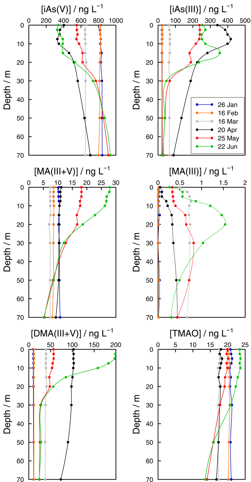
Fig. 6 Vertical profiles of As species ( \text{iAs(V)} , \text{iAs(III)} , \text{MA(III + V)} , \text{MA(III)} , \text{DMA(III + V)} , and \text{TMAO} ) concentrations in the Petit Lac (point GE3) from January to June 2021.
