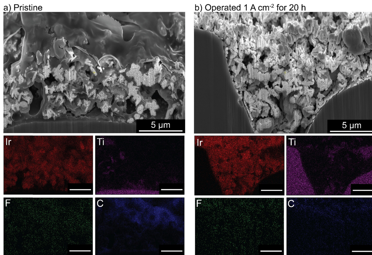
Fig. 5 Cross-sectional imaging and EDX of IrO x /20% TP-85 anode PTE. (a) Before and (b) after 20 h operation at 1 A cm -2 . All scale bars are 5 μm. No ionomer is observed in the catalyst layer after operation.
