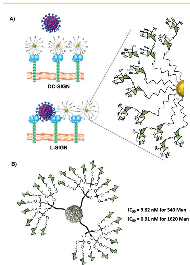
Fig. 8 (A) Schematic representation of the interaction of \text{Man}\alpha 1,2\text{Man} glycoAuNP with the four binding sites of DC-SIGN inhibiting DC-SIGN-dependent viral infection and cross-linking with some binding sites or L-SIGN allowing the virus interaction with unblocked L-SIGN binding sites. (B) General structure of mannosylated glycodendron VLPs functionalised with 540 and 1620 mannose units and their corresponding \text{IC}_{50} values.
