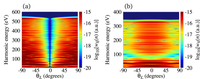
Fig. 6 Logarithm of the harmonic emission rate of the \text{C}_2^+ [(panel (a))] and \text{Li}_2^+ [(panel (b))] cations, exposed to a linearly polarised field, as a function of the harmonic energy and the orientation angle \theta_L . The results for the \text{C}_2^+ cation are obtained using the laser field with the same parameters as in Fig. 2, while the results for the \text{Li}_2^+ cation correspond to a linearly polarised field with the intensity I = E_1^2 = 6 \times 10^{13} \text{ W cm}^{-2} and the wavelength of 2800 nm.
