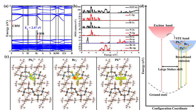
Fig. 4 (a) Calculated electronic band structures and (b) DOS of (HM)Pb 2 Br 6 . (c) Calculated charge density for (HM)Pb 2 Br 6 (Pb 2 3+ STLs, Br 2 - and Pb 3 + STLs holes) upon crystal lattice perturbation via the Pb-Pb, Br-Br and Pb-Br distances shortening. (d) Configuration coordinate diagram illustrating the luminescence mechanism.
