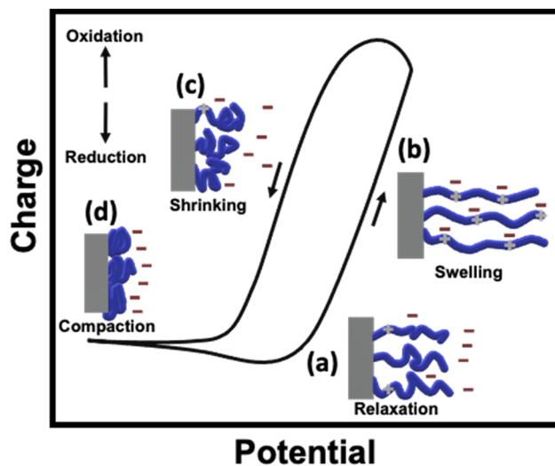
Fig. 1 Characteristic coulombic voltammogram obtained during the charging/discharging process of a neutral and partially de-doped polymer with a schematic representation of the different conformational changes within the polymeric matrix: (a) relaxation, (b) swelling, (c) shrinking and (d) compaction.
