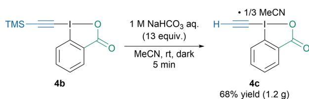
Scheme 5 Synthesis of EBX-MeCN complex 4c .
