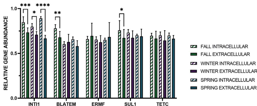
Fig. 3 Relative gene abundance of the intracellular and extracellular fraction of int11 , bla TEM , ermF , sul1 , and tetC in stormwater samples normalized to the i -16S rRNA and e -16S rRNA genes, respectively. The asterisk indicates a statistically significant relationship between the intracellular and extracellular relative concentrations (Student's t -test, p -value < 0.05) and the error bars represent the standard deviation of the mean ( n = 12).
