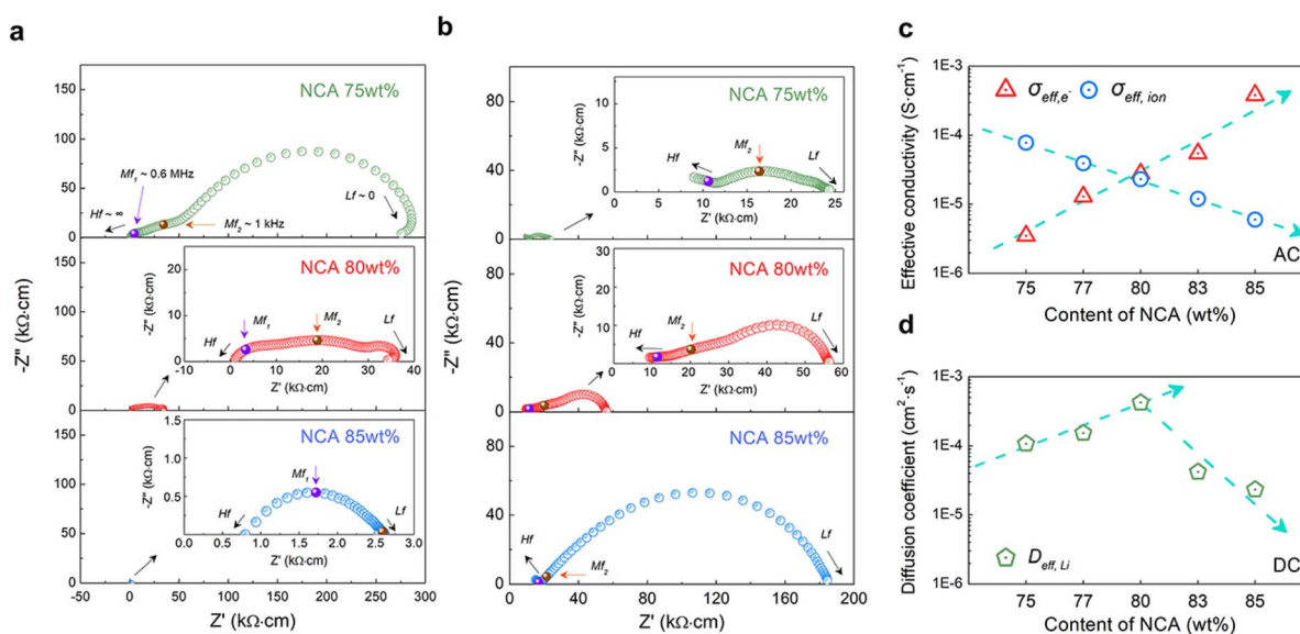
Fig. 4 Nyquist plots of (a) ion-blocking cells [SS||composite cathode||SS] and (b) electron-blocking cells [Li]||LPSC||composite cathode||LPSC||[Li] with 75 wt%, 80 wt%, and 85 wt% of NCA in composite cathodes. (c) Effective conductivity ( \sigma_{\text{eff}} ) and (d) diffusion coefficients ( D_{\text{eff},Li} ) results of the composite cathode extracted from EIS and DC polarization measurements as a function of NCA content from 75 wt% to 85 wt%.
