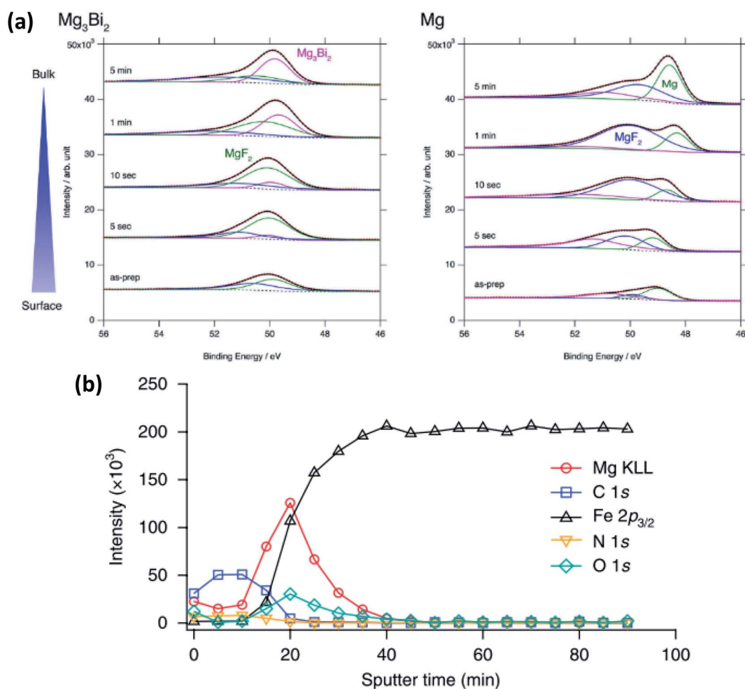
Fig. 18 (a) Mg 2p XPS spectra after sputter-etch depth profiling for \text{Mg}_3\text{Bi}_2 and Mg thin films immersed in 0.5 mol \text{L}^{-1} \text{Mg}(\text{TFSA})_2 in \text{BuMeG3} solution for 24 h. Reproduced under CC-BY licence from ref. 155. (b) XPS sputter-etch depth profiles of a Mg-coated stainless-steel electrode in 0.5 M \text{Mg}(\text{TFSI})_2 -PC electrolyte. Reprinted by permission from Nature Chemistry 156 Copyright 2018.
