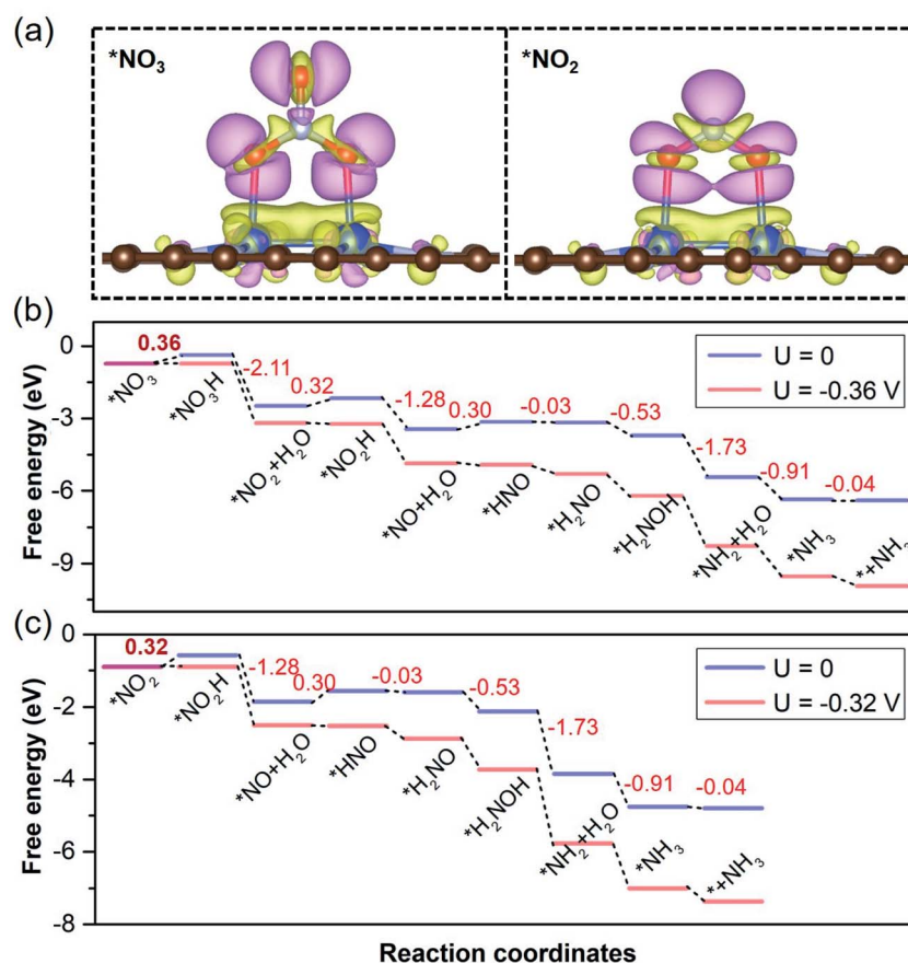
Fig. 6 (a) The most stable configurations with the CDD ( 0.002 \text{ e } \text{\AA}^{-3} ) for *NO_3 and *NO_2 over the Cu_2 DAC. The purple and yellow maps in the CDD denote electron accumulation and depletion, respectively. (b) The free energy diagrams for the NO_3RR towards NH_3 over the Cu_2 DAC. (c) The free energy diagrams for the NO_2RR towards NH_3 over the Cu_2 DAC. In (b) and (c), the corresponding free energy changes of the key steps along the reaction pathway are presented and the \Delta G_{max} values of PDS are in bold.
