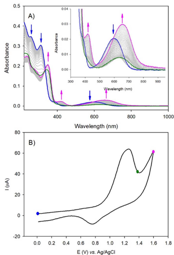
Fig. 6 UV-vis-NIR spectroelectrochemistry of ( \mathbf{1}(\text{O}_A)_x(\text{C})_z ), ( c = 1.72 \times 10^{-4} M, 20 °C) upon electrochemical oxidation in 0.1 M n -Bu 4 NPF 6 in acetonitrile/1,4-dioxane (1/1) solution at a scan rate of 20 mV s -1 . (A) Evolution of the UV-vis-NIR spectra recorded during oxidation. Optical path length = 0.02 cm. (B) CV at a scan rate of 20 mV s -1 recorded during the spectroelectrochemistry measurement. Note that the start of the recording (blue curve) is done when the equilibrium from closed to open form is reached under UV-visible illumination.
