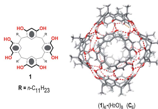
Fig. 1 Chemical drawing of C-undecylresorcin[4]arene 1 (left) and a reduced model ( R = Me ) of the hexameric capsule (1)_6 \cdot (H_2O)_8 ( C_6 ) (right).
