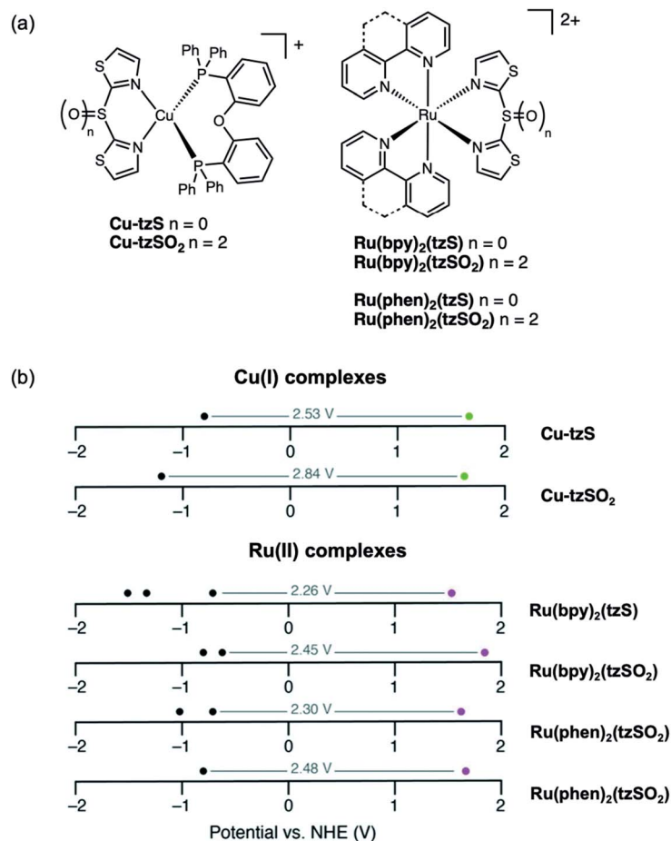
Fig. 19 (a) Structures of \text{Cu-tzSO}_n and \text{Ru}(\text{bpy})_2(\text{tzSO}_n) and \text{Ru}(\text{phen})_2(\text{tzSO}_n) complexes reported by our group ( n = 0, 2 ). (b) Redox potentials of Cu(I) and Ru(II) complexes with reductive (black dots) and oxidative (green or purple dots) potentials illustrated. Adapted with permission from ref. 95. Copyright 2019 Royal Society of Chemistry.
