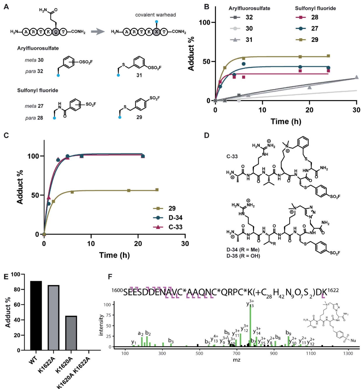
Fig. 5 Design and biochemical evaluation of covalent peptides targeting the PHD3 domain. (A) H3K4me3 6mer peptides bearing covalent lysine-reactive warheads. (B) PHD3 (10 \mu\text{M} ) was treated with peptides 27–32 at 50 \mu\text{M} , and the extent of labelling was monitored over time by intact protein LCMS. (C) Comparison of cross-linking efficiency between linear (29) and cyclic (C-33 and D-34) peptides. (D) Structures of covalent cyclic peptides C-33, D-34, and D-35. (E) Comparison of peptide-PHD3 adduct formation between WT and mutant PHD3 after 5 h incubation time. Triazole probe D-35 was used for this experiment. (F) HCD product ion spectrum of the triazole probe (D-35)-labeled PHD3 domain following tryptic digestion, corresponding to precursor ion at m/z = 678.8795^+ . C* indicates carbamidomethylated Cys. The structure of the probe adduct following digestion is shown and the spectrum indicates K1620 as the site of modification.
