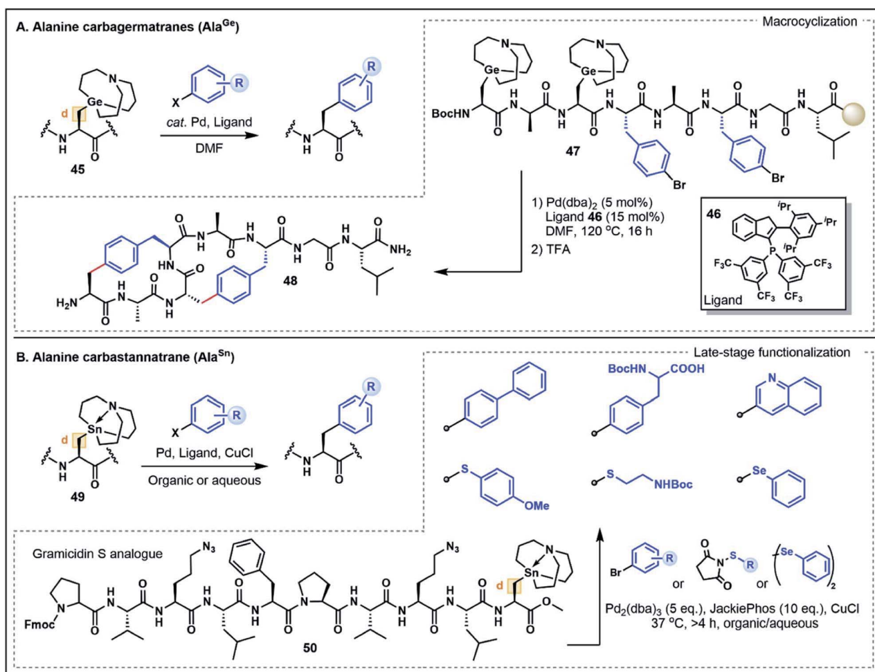
Fig. 7 Ala umpolung strategies. (A) Overview of Ala carbagermatrane derivatives and their use in peptide macrocyclization. (B) Overview of Ala carbastannatran derivatives and their applications in late-stage functionalization.
