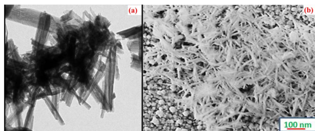
Fig. 22 (a) TEM (b) SEM images of the Cu 2 O grains showing needle-shaped uniformity on the surface. 146
