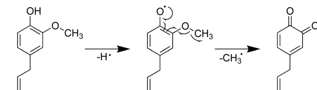
Scheme 2 Mechanism for the reaction between eugenol and ROO • .
