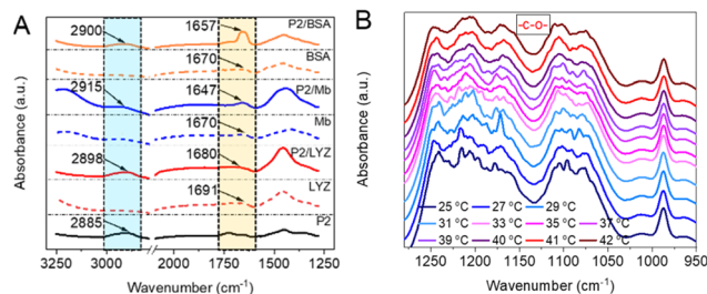
Fig. 3 FT-IR spectra of (A) PG1/protein , free proteins, and PG1 , at 25 °C (the different colour areas are a guide for the eye), and (B) PG1S-Mb at different temperatures. All samples were prepared in D 2 O.
