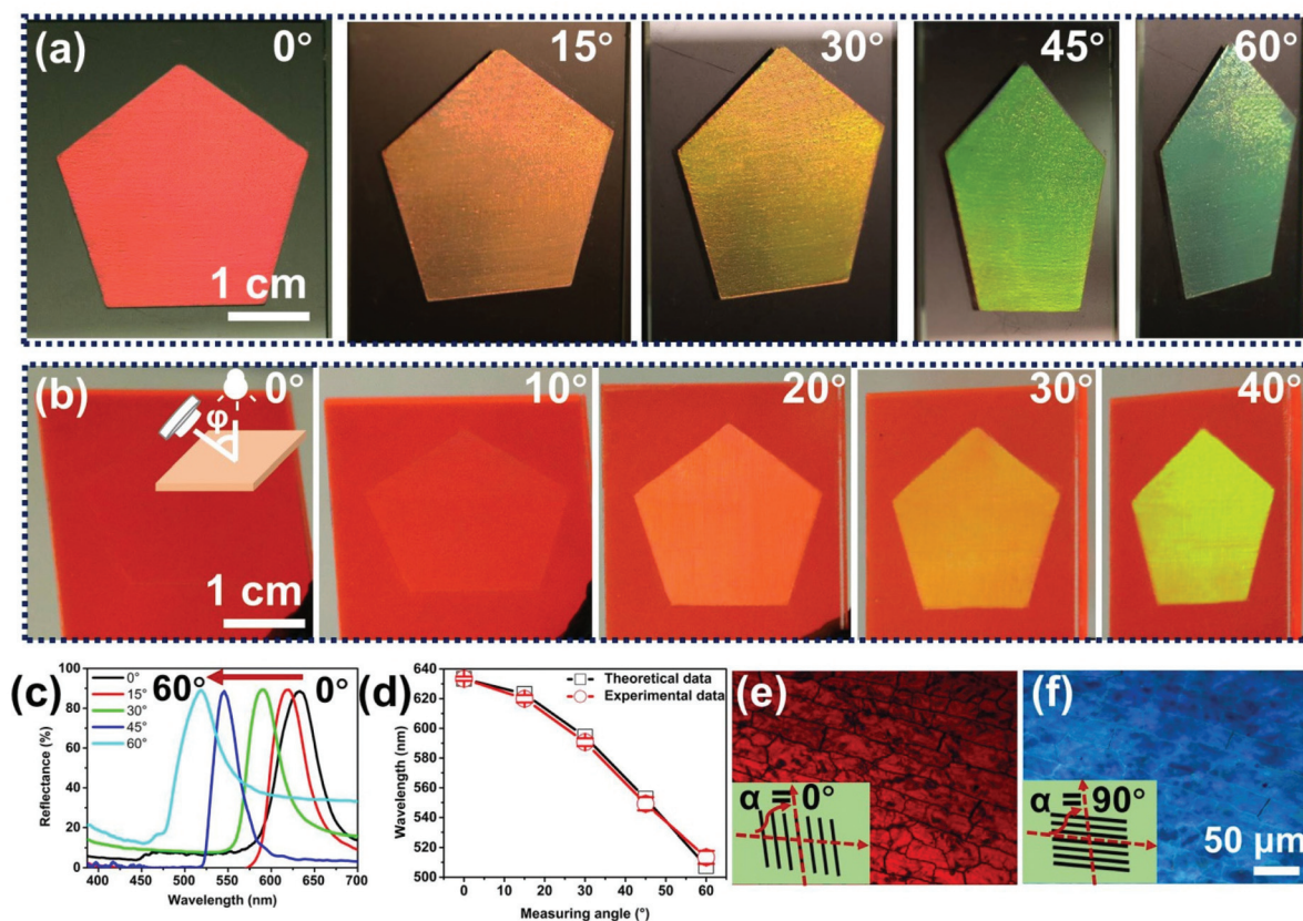
Fig. 2 Optical properties of colloidal crystal films with PUFs. (a) A typical colloidal crystal film with the pentagon pattern changed its structural color from red to cyan at viewing angles from 0° to 60°. (b) The angle-dependent structural-colors of the colloidal crystal film enabled the hiding and revealing of the pentagon patterns on a red plastic substrate. The inset indicates the relative positions of the light source, sample and camera. (c) The reflectance spectra of the red pentagon pattern colloidal crystal film at testing angles from 0° to 60°. (d) The dependence of the reflectance peaks on the testing angles (black line, theoretical data and red line, experimental data). (e) and (f) Cross-polarized optical microscopy images of the colloidal crystal films at 0° and 90°. The color of the film changed to blue due to the polarization anisotropy of the crystal structure.
