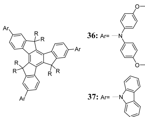
Scheme 14 Examples of electron-rich truxenes.
