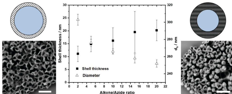
Fig. 3 Influence of alkyne:azide ratio on the shell thickness (■) and diameter ( \Delta ) of protein nanocarriers. Scanning electron micrographs of HSA nanocarriers using a 2:1 (left) and 20:1 (right) ratio (Scale bar: 0.5 \mu\text{m} ).
