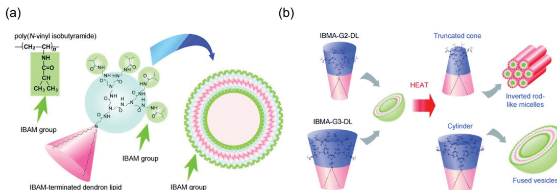
Fig. 10 (a) Design of molecular assemblies with temperature-sensitive properties using isobutyramide terminated dendron-based lipids. (b) Mechanism for temperature-responsive structural transition. Reprinted with permission from ref. 128. Copyright 2011, WILEY-VCH.
