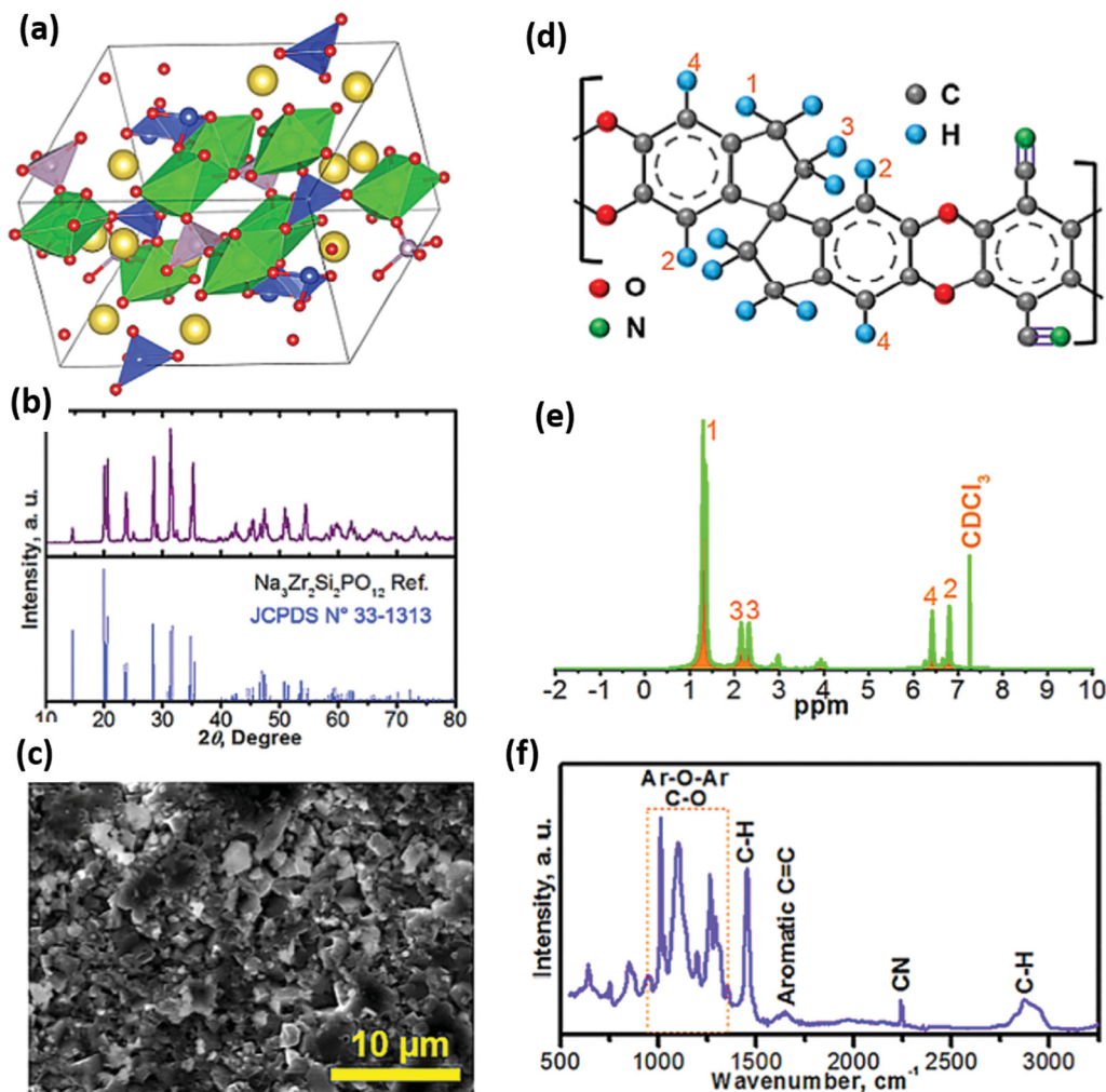
Fig. 8 Various characterization methods of the Na 3 Zr 2 Si 2 PO 12 solid electrolyte and the intrinsic nano-porous polymer (a) schematic representation of the structure of NASICON, (b) overlaid XRD of Na 3 Zr 2 Si 2 PO 12 membrane and Na 3 Zr 2 Si 2 PO 12 reference XRD pattern, (c) SEM image showing the dense structure of Na 3 Zr 2 Si 2 PO 12 , (d and e) chemical structure of the polymer and corresponding 1 H-NMR spectrum, (f) FTIR spectrum with bands showing various stretching/bending vibrations for the polymer. 72
