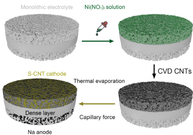
Fig. 9 Schematic representation of depositing nickel nitrate (Ni(NO 3 ) 2 ) solution and chemical vapor deposited CNT over monolithic electrolyte with the cell architecture of a solid-state RT Na-S battery. 129
