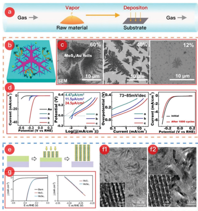
Fig. 2 (a) Schematic of the CVD process. (b) Schematic of the dendritic \text{MoS}_2/\text{Au} foil. (c) SEM images of each \text{MoS}_2/\text{Au} sample with \text{MoS}_2 coverages of 60%, 40%, and 12%, named a, b, and c, respectively. (d) Electrochemical performances of samples for HER. (The images of (b–d) were reproduced with permission. Copyright 2014, American Chemical Society, ref. 119.) (e) Schematic of the synthesis mechanism of \text{MoS}_2/\text{Mo} or \text{MoSe}_2/\text{Mo} . (f1) SEM image of the \text{MoS}_2/\text{Mo} sample. (f2) SEM image of the \text{MoSe}_2/\text{Mo} sample. (g) HER catalytic performance of both \text{MoS}_2/\text{Mo} electrode and \text{MoSe}_2/\text{Mo} electrode. (The images of (e–g) were reproduced with permission. Copyright 2013, American Chemical Society, ref. 117.)
