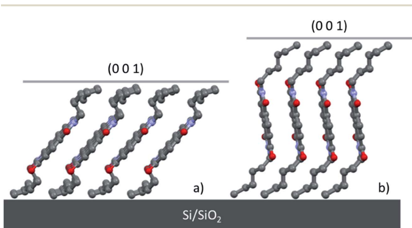
Fig. 9 Molecular arrangement of thin films oriented in the \text{Si/SiO}_2 substrates of (a) Form \alpha and (b) Form \gamma .
