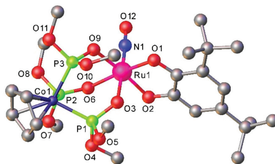
Fig. 8 X-ray diffraction structure of [Ru(L OMe )(NO)(cat)] complex, where cat = dianion of 3,5-di- tert -butylcatechol, L OMe = [CpCoP(O)(OMe) 2 ] 2 3- . The structure is taken from those reported on the CSD; code: CALXAR.
