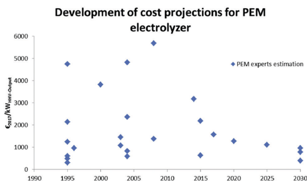
Fig. 165 Cost projections for alkaline and PEM electrolyzers surveyed from the literature. Reproduced from Saba et al. 1923
