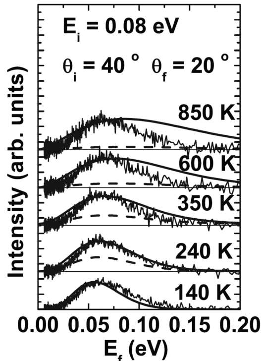
Fig. 4 Energy-resolved spectra, scattered intensity versus final energy, of Ar scattered from Ru(0001) with an incident energy of 0.08 eV and temperatures ranging from 140 to 850 K as marked. The incident and final polar angles are \theta_i = 40^\circ and \theta_f = 20^\circ . Theoretical calculations are shown as solid curves and the dashed curves indicate the calculated intensities relative to that at T = 140 K. (Reprinted with permission from ref. 73, Copyright [2002] Royal Chemistry Society.)
