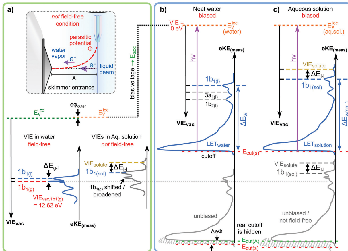
Fig. 8 (a) Top: Depiction of potential drop between charged liquid jet (LJ) and grounded electron detector. Horizontal arrows indicates that photoelectrons from water gas-phase ionization gain different energy in the resulting electric field gradient than photoelectrons from the liquid surface, resulting in different measured eKEs depending on the distance of origin from detector/jet. Bottom, right: Valence liquid-water jet photoelectron spectrum measured with the 'Gas-Phase Method' (see main text) under non-field-free conditions, i.e. , in presence of parasitic potentials, which is usually the case. Under these conditions VIE_{1b_1(g)} is not a reliable energy reference. Bottom, left: Valence liquid-water jet photoelectron spectrum measured with the 'Gas-Phase Method' under field-free conditions, i.e. , where the solution and experimental conditions have been precisely tuned to eliminate all potentials. This leads to a sharp water 1b_1 gas-phase peak, and correct peak separation from the liquid-phase 1b_1 peak, such that \Delta E = VIE_{1b_1(g)} - VIE_{1b_1(l)} yields the accurate VIE_{1b_1(l)} value, and VIE_{1b_1(g)} being the known literature value; see main text. (b) Left: A bias voltage applied to the LJ shifts all liquid features under the influence of an accelerating field, E_{acc} (blue spectrum); the gas-phase PE signal is smeared out and does not appear here. Biasing reveals the full LET curve and cutoff energy of the sample spectrum. Without bias (grey spectrum), the real cutoff is obscured by the work-function difference between the liquid and analyzer, \Delta E_{\Phi} . E_{cut} constitutes a low-energy limit for photoelectrons to still overcome the liquid-surface barrier, and is thus connected to the local vacuum level above the LJ surface, E_{loc,v} . The precisely known photon energy, h\nu (vertical purple arrow) is used to map E_{loc,v} onto the measured spectrum and define the VIE_{vac} scale. Thus, with the knowledge of h\nu and the energetic distance of a peak feature to the cutoff, \Delta E_w , the accurate VIE of this feature can be determined. (c) As for (b) but for an arbitrary aqueous solution; here, the spectra are arbitrarily aligned to the cutoff, which at the same time aligns E_{loc,v} . Changes in \Delta E_w directly translate to changes in the VIE. The lower part of this panel shows the full unbiased spectrum (compare to the spectra shown in panel A and bottom part of panel B). Fig. 8 is adapted from Fig. 1 of ref. 22
