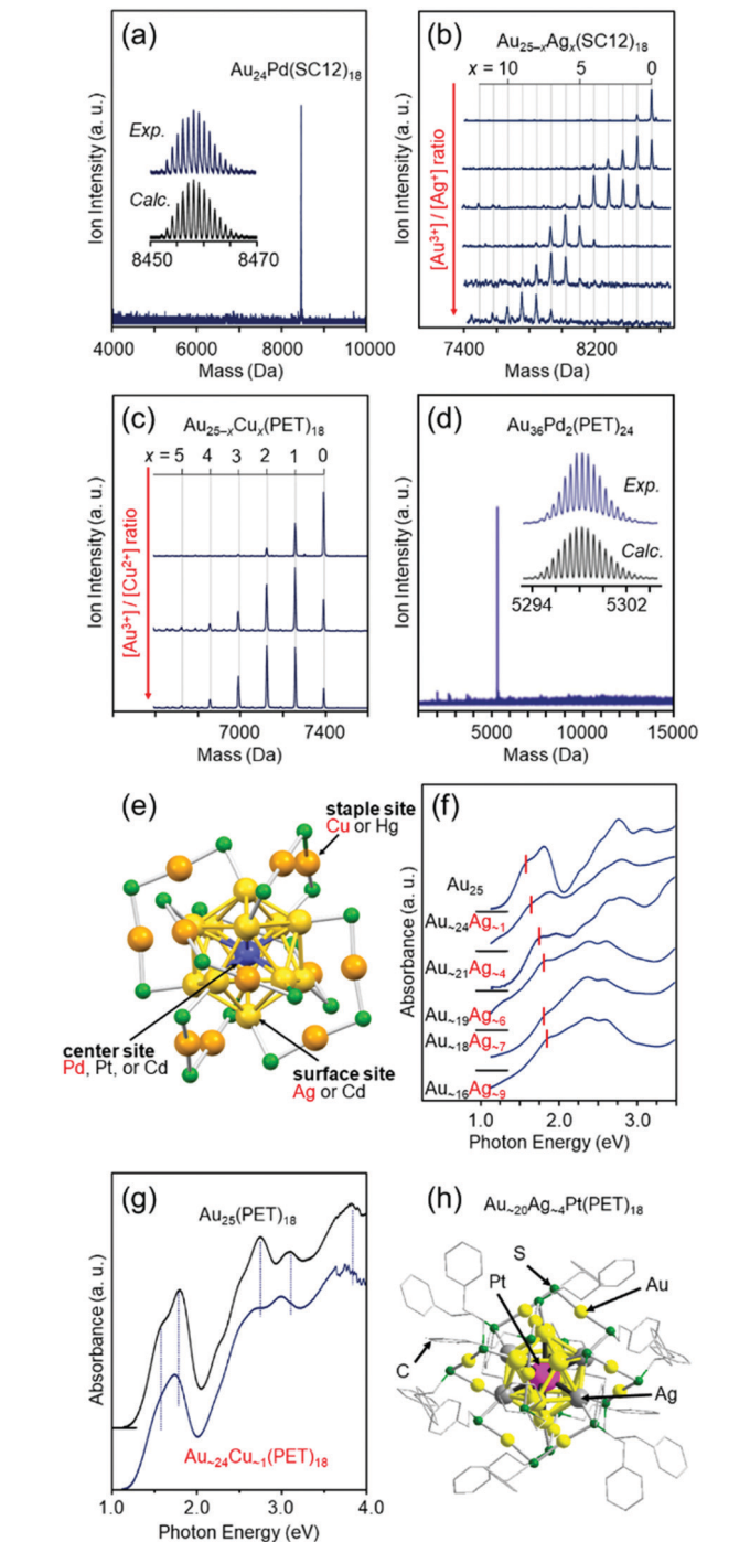
Fig. 6 Negative-ion MALDI mass spectra of (a) Au_{24}Pd(SC12)_{18} , 110 (b) Au_{25-x}Ag_x(SC12)_{18} , 111 and (c) Au_{25-x}Cu_x(PET)_{18} . 112 (d) Negative-ion ESI mass spectrum of Au_{36}Pd_2(PET)_{24} . 114 (e) Preferential substitution site in Au_{25}(SR)_{18} for each element. 116 Blue, yellow, and orange spheres represent Au atoms, and green spheres represent S atoms. The R groups are omitted for clarity. Optical absorption spectra of (f) [Au_{25-x}Ag_x(SC12)_{18}]^- and (g) [Au_{25-x}Cu_x(PET)_{18}]^- . 112,158 (h) Geometric structure of [Au_{20}Ag_4Pt(PET)_{18}]^0 . 117 Reproduced with permission from ref. 110–112, 114, 116 and 117. Copyright 2010 The Royal Society of Chemistry, 2012 American Chemical Society, 2012 The Royal Society of Chemistry, 2016 The Royal Society of Chemistry, and 2018 American Chemical Society.
